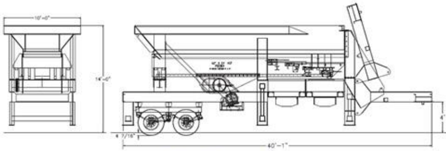
Travel Dimensions
