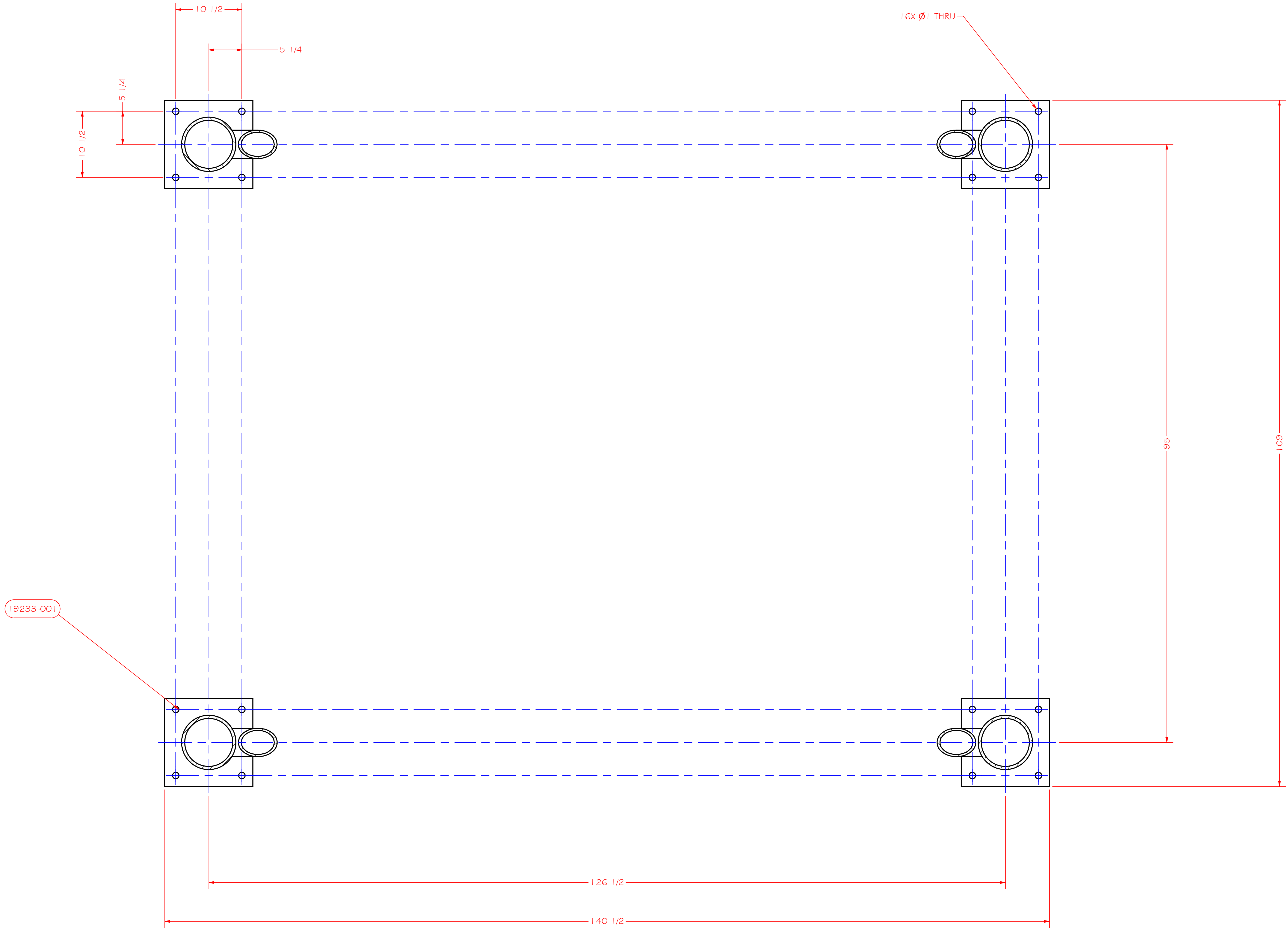
SECTION A-A SCALE 1 1/2" = 1'-0"
