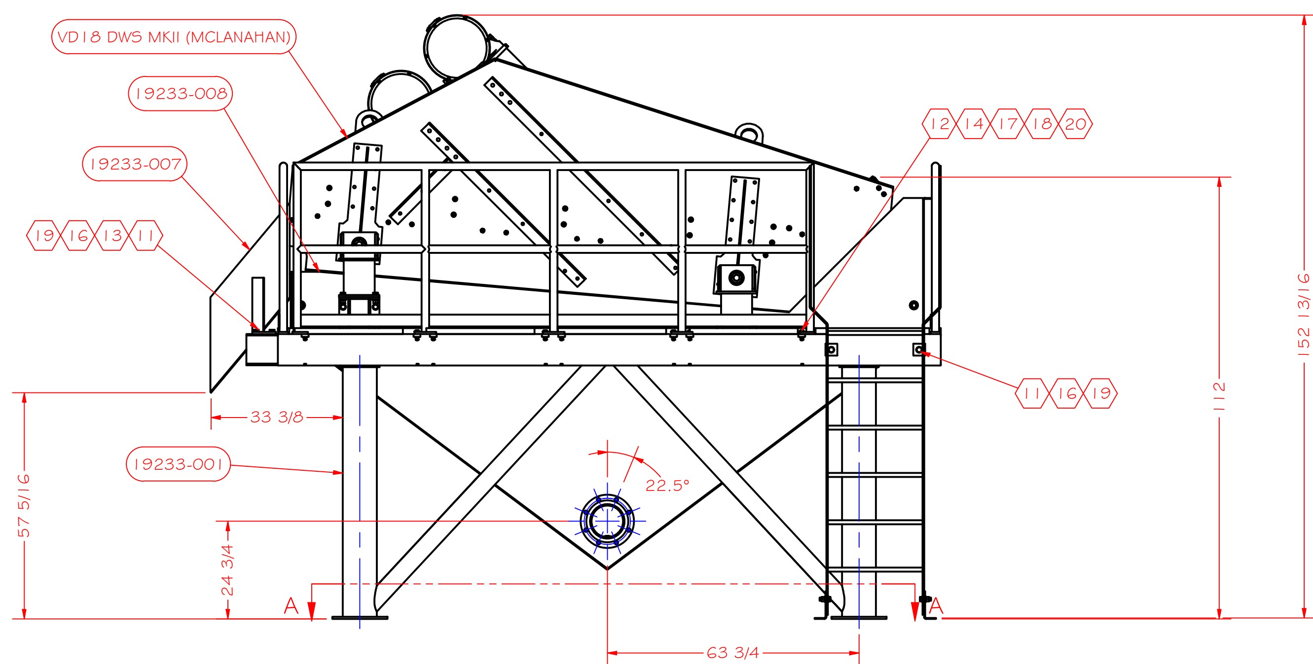
PCS MK - 19233 6' DWS STRUCTURE, DISCHARGE CHUTE, UNDERPAN SCALE 1/2" = 1'-0"
