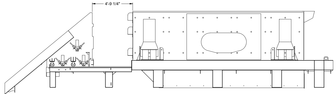
SIDE VIEW: ROLL AWAY CHUTE OPEN
