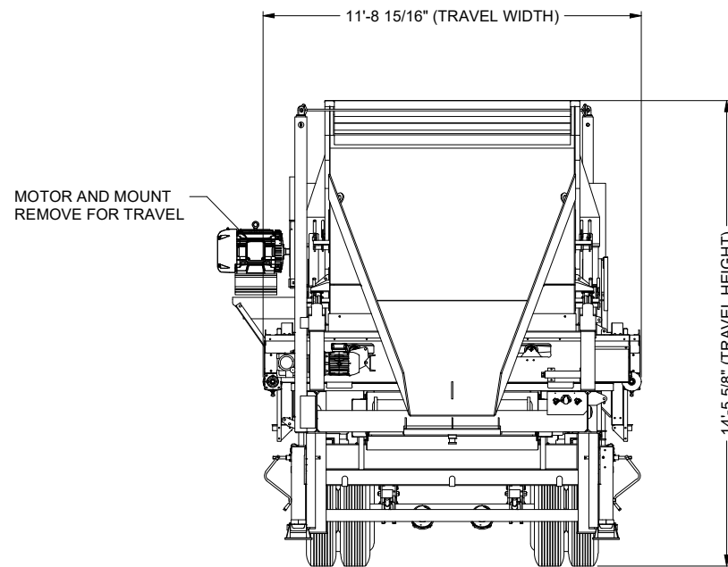
FRONT VIEW: TRAVEL MODE
